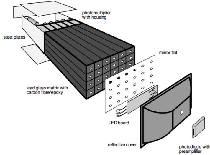
Figure 2.19: A diagram illustrating the construction of a PbG1 supermodule.
