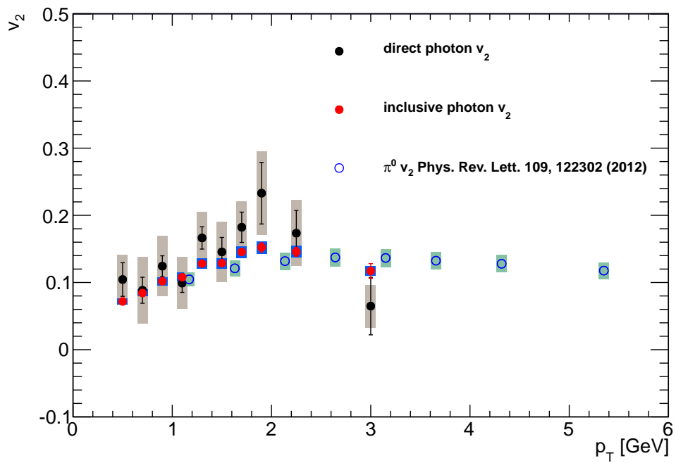
Figure 7.3: A comparison of the v_2^{direct} , v_2^{incl} and v_2^{\pi^0 decay} .
