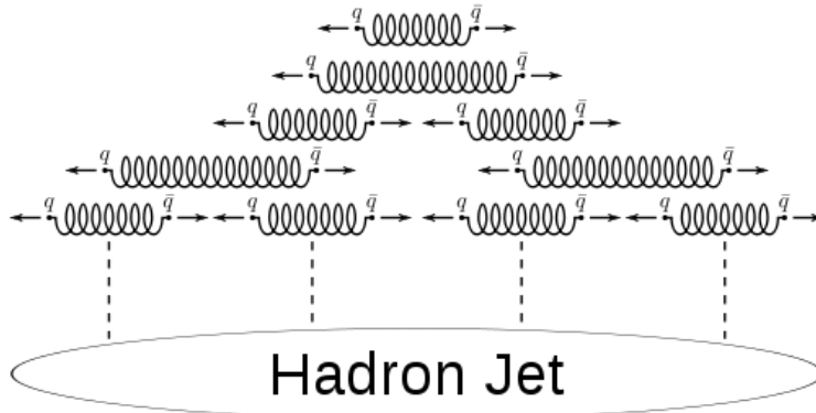
Figure 1.2: A cartoon illustrating quark confinement. The top row depicts a q\bar{q} pair moving away from each other. As they move apart, the flux tube connecting them gets longer, indicating an increase in potential energy. Eventually it becomes more energetically favorable for the tube to break to form a new q\bar{q} pair, closing the open ends of the broken flux tubes, and resulting in two lower energy tubes. This process continues until it is no longer energetically favorable to do so.
