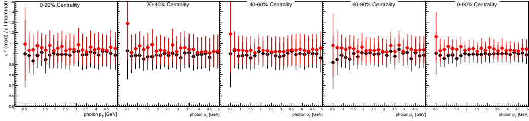
Figure 4.30: The systematic uncertainty of the energy scale mismatch in data and simulation shown in each centrality bin as a ratio of the correction with the energy cut off up and down by 2% to the correction with the nominal energy cut. A flat ratio of 4% is taken as the systematic uncertainty independent of p_T and centrality.
