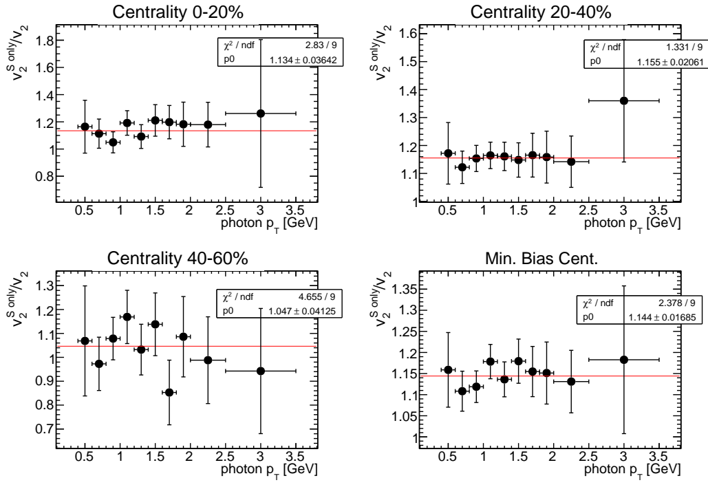
Figure 6.11: The ratio of the south detector only v_2 to the north plus south v_2 . A constant shift is observed in each centrality.
